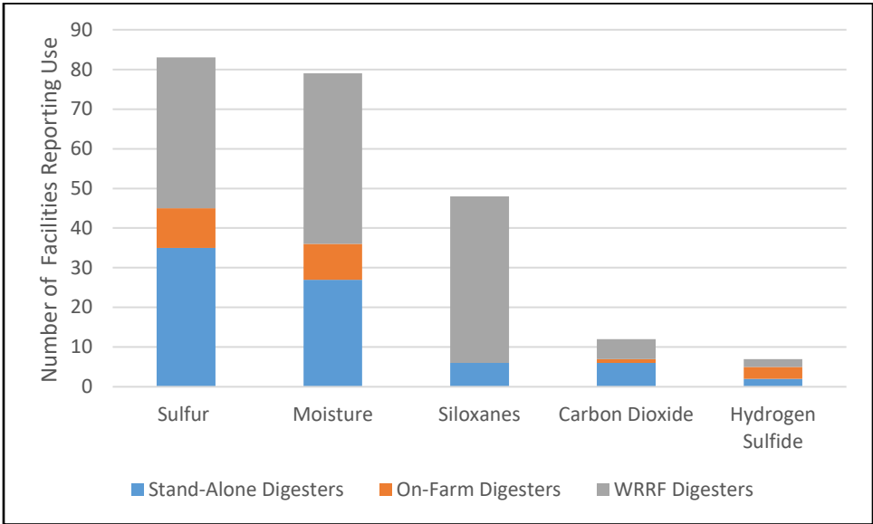
Figure 9: Top Five Constituents Removed by Digester Type (2015)
